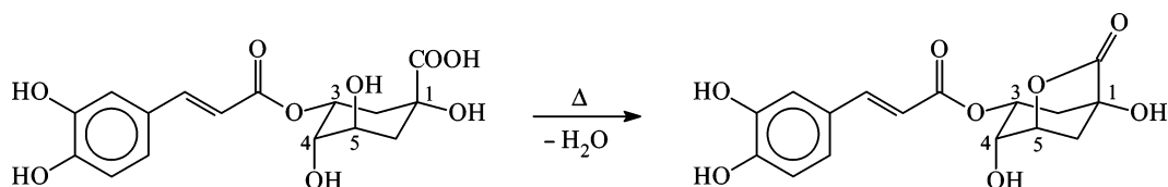
Figure 2. Formation of a cinnamoyl-1,5- \gamma -quinolactone from a chlorogenic acid isomer. Although under IUPAC rules (16) the numbering system for the lactones is different from that for the acids, to avoid confusion, in this work, we have used for lactones the same numbering of the carbons as for their precursors. When other authors are cited, the numbering has been changed for consistency.
